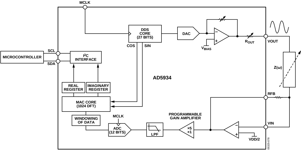
Figure 14. Block Overview
