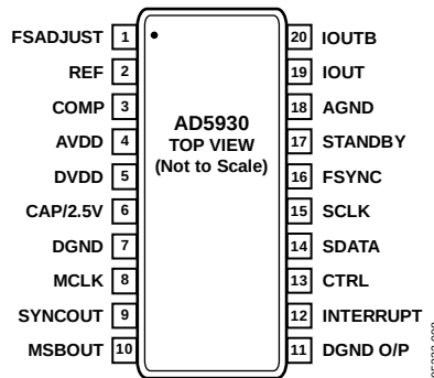
Figure 8. Pin Configuration
