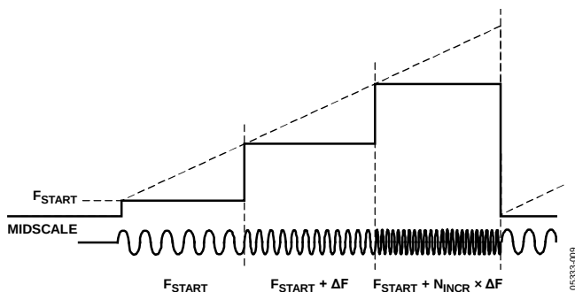
Figure 31. Saw-Sweep Profile
