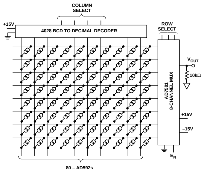
Figure 16. Matrix Multiplexer
