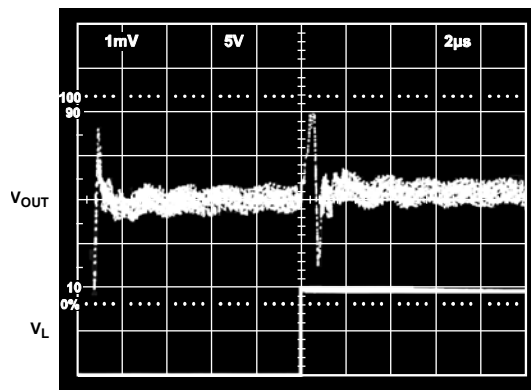
Figure 28. Load Crosstalk
