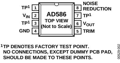
Figure 2. Pin Configuration (N-8)
