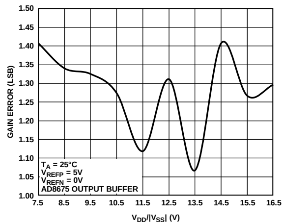
Figure 26. Gain Error vs. Supply Voltage, 5 V Span
