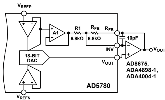
Figure 53. Output Amplifier in Gain-of-Two Configuration
