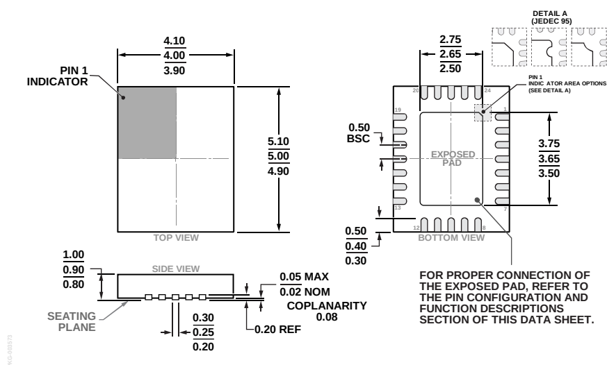
Figure 55. 24-Lead Lead Frame Chip Scale Package [LFCSP] 4 mm × 5 mm Body and 0.90 mm Package Height (CP-24-5)
