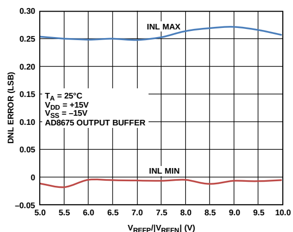
Figure 28. Differential Nonlinearity Error vs. Reference Voltage
