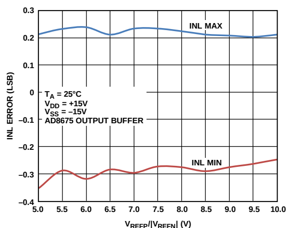
Figure 27. Integral Nonlinearity Error vs. Reference Voltage
