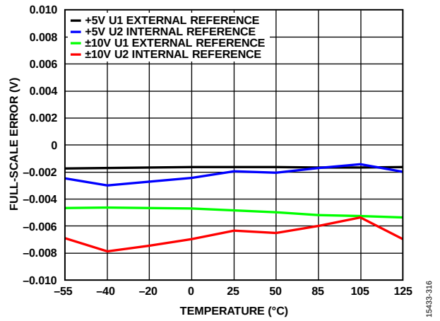
Figure 8. Full-Scale Error vs. Temperature
