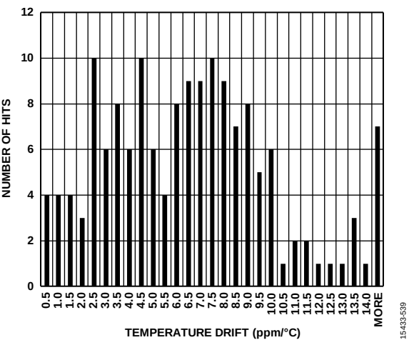
Figure 12. Reference Output TC
