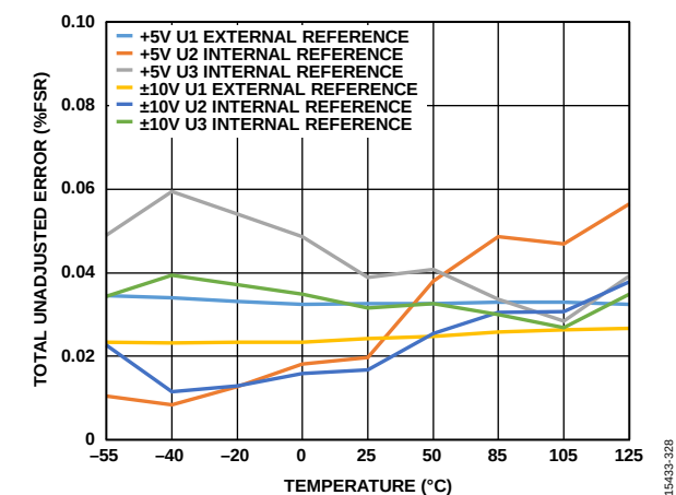
Figure 10. Total Unadjusted Error (TUE) vs. Temperature
