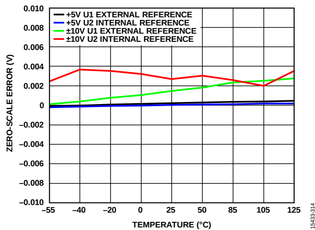
Figure 6. Zero-Scale Error vs. Temperature
