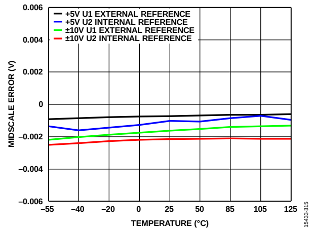
Figure 7. Midscale Error vs. Temperature
