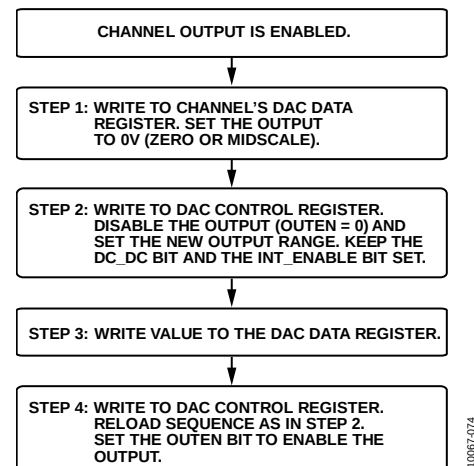
Figure 51. Programming Sequence to Change the Output Range
