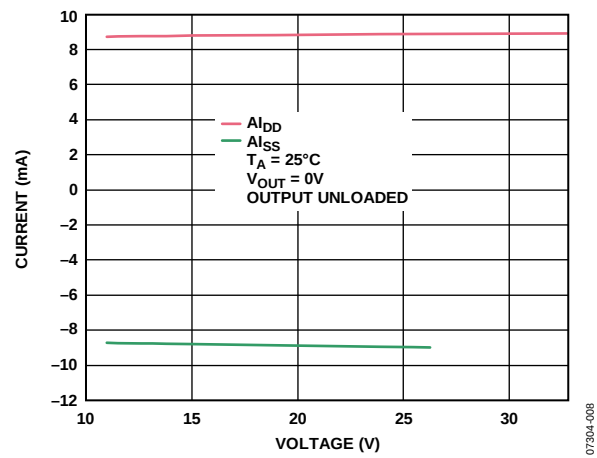
Figure 67. A_{DD}/A_{SS} vs. A_{VDD}/A_{VSS}
