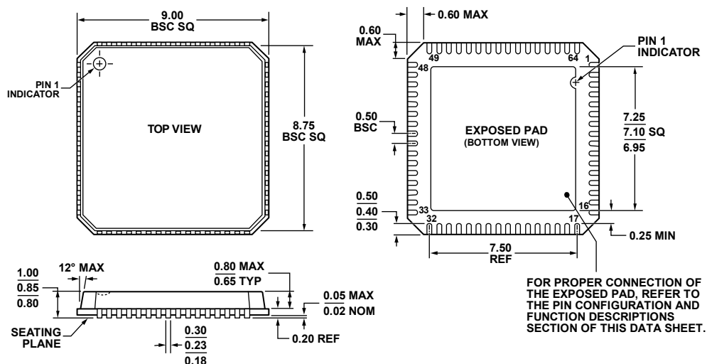
Figure 87. 64-Lead Lead Frame Chip Scale Package [LFCSP_VQ]
