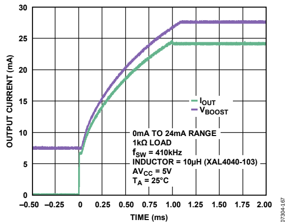
Figure 48. Output Current and V_{BOOST,x} Settling with DC-to-DC Converter (See Figure 78)
