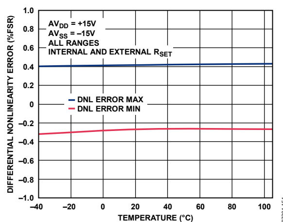
Figure 36. Differential Nonlinearity vs. Temperature
