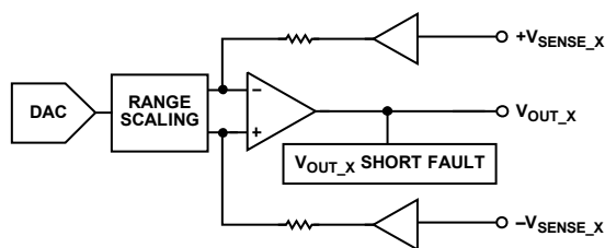
Figure 71. Voltage Output
