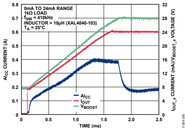
Figure 81. A_{Icc} Current vs. Time for 24 mA Through 1 kΩ Slew with External 51 kΩ Compensation Resistor
