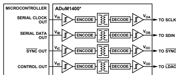
Figure 86. Isolated Interface
