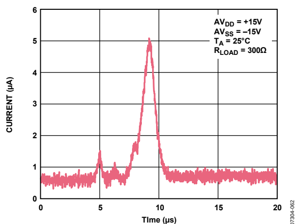
Figure 46. Output Current vs. Time on Power-Up
