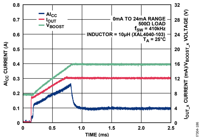
Figure 82. A_{Icc} Current vs. Time for 24 mA Through 500 Ω Slew with External 51 kΩ Compensation Resistor
