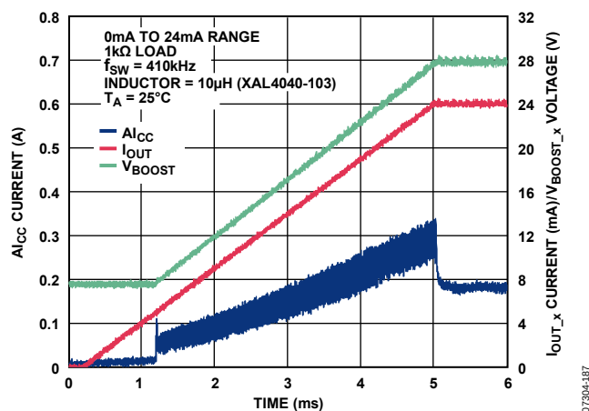
Figure 83. A_{Icc} Current vs. Time for 24 mA Slew with Slew Rate Control
