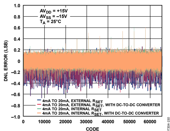
Figure 32. Differential Nonlinearity vs. Code
