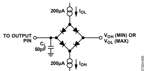
Figure 6. Load Circuit for SDO Timing Diagram
