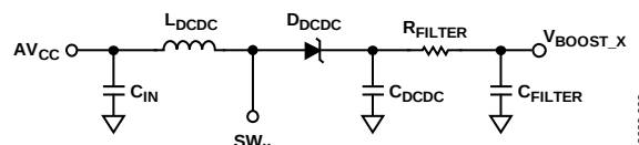
Figure 4. DC-to-DC Converter Circuitry
