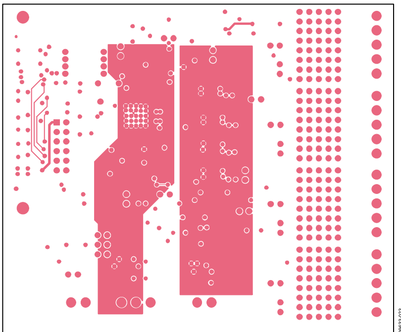
Figure 25. Inner Second PCB Layer
