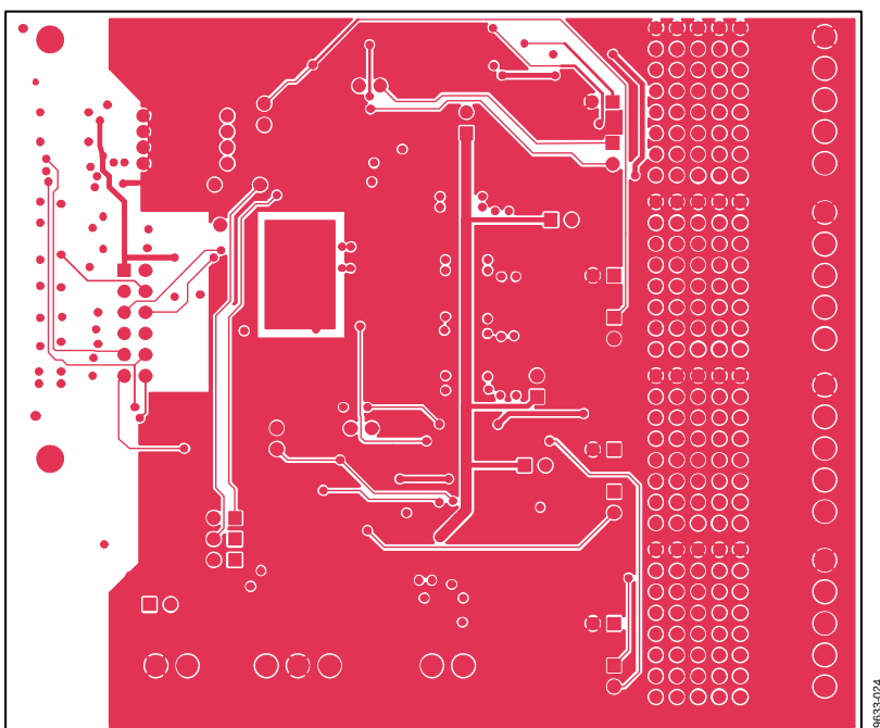
Figure 26. Bottom PCB Layer
