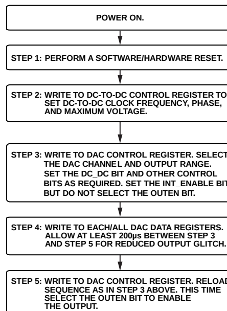
Figure 9. Programming Sequence for Enabling the Output Correctly
