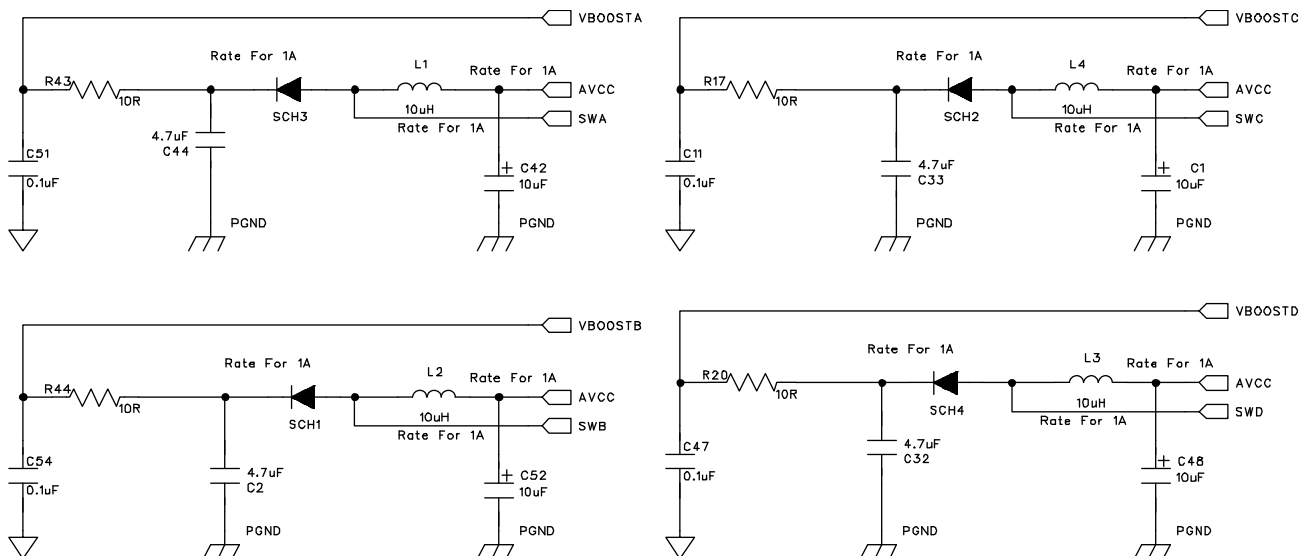
Figure 18. DC-to-DC Circuitry
