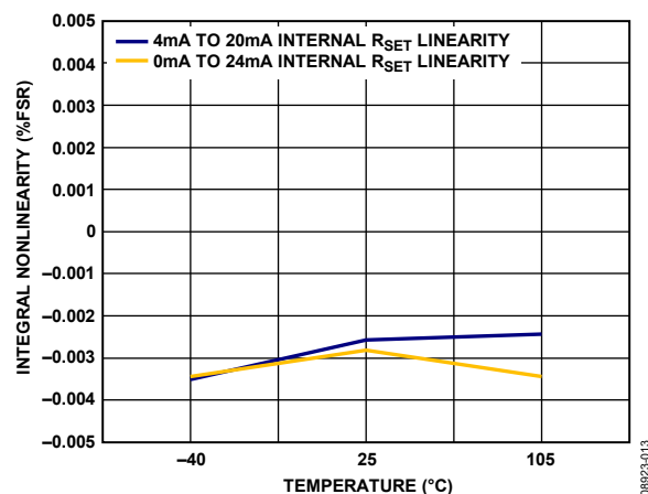
Figure 13. Integral Nonlinearity Error vs. Temperature, Internal R_{SET} Sense Resistor
