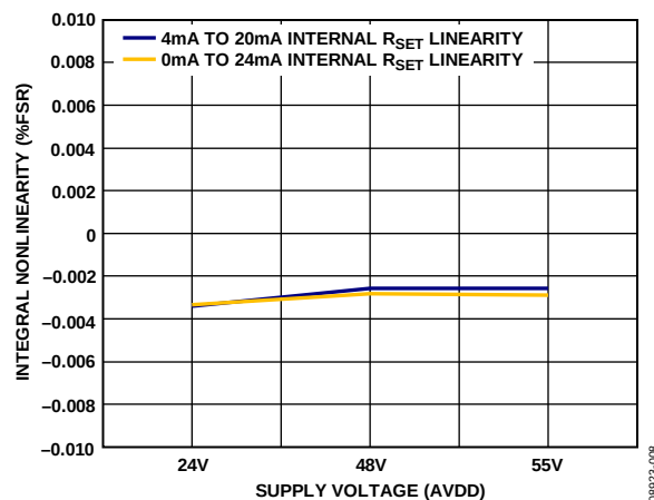
Figure 8. Integral Nonlinearity Current Mode, Internal R_{SET} Sense Resistor
