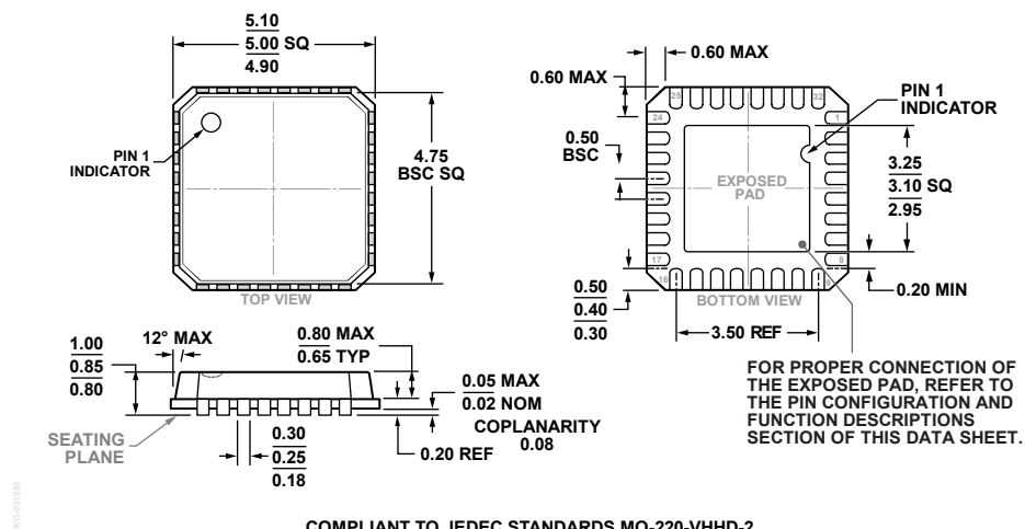
Figure 38. 32-Lead Lead Frame Chip Scale Package [LFCSP] 5 mm × 5 mm Body and 0.85 mm Package Height (CP-32-2) Dimensions shown in millimeters
