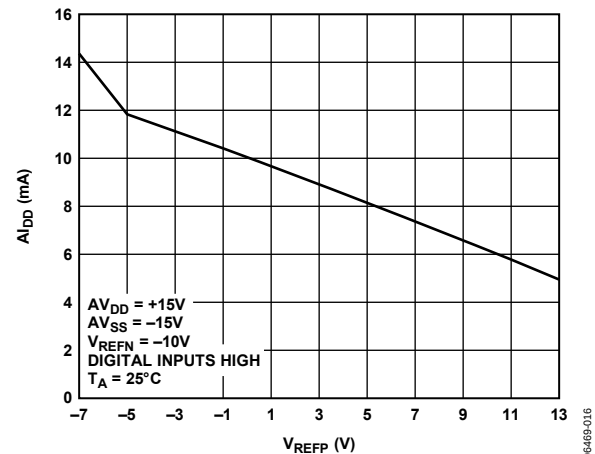
Figure 17. A_{IDD} vs. V_{REFP} , All DACs Loaded with Full-Scale Code
