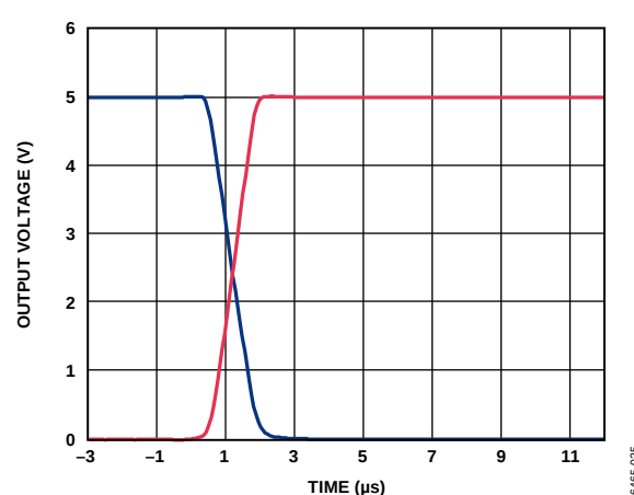
Figure 28. Full-Scale Settling, +5 V Range
