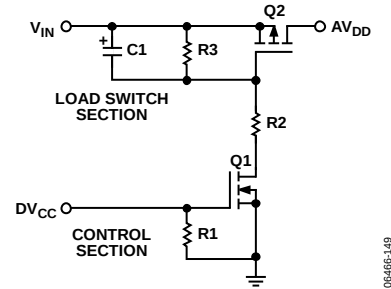
Figure 49. Load Switch Control Circuit
