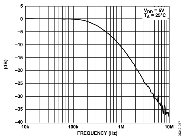
Figure 51. Multiplying Bandwidth
