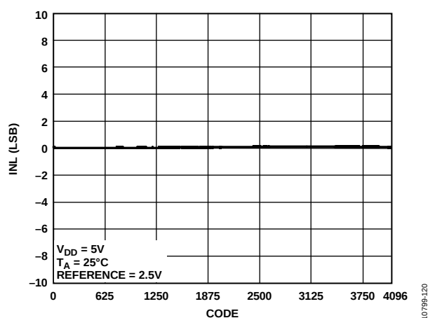
Figure 6. AD5694 INL
