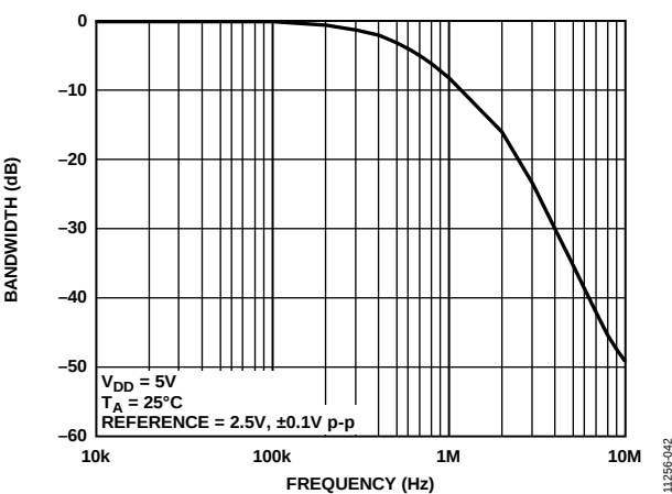
Figure 40. Multiplying Bandwidth, External Reference = 2.5 V, ±0.1 V p-p, 10 kHz to 10 MHz
