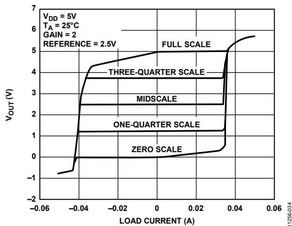
Figure 32. Source and Sink Capability at 5 V, Gain = 2
