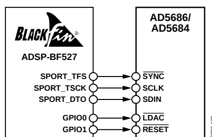
Figure 44. SPORT Interface
