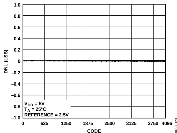
Figure 11. AD5684 DNL
