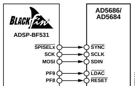
Figure 43. ADSP-BF531 Interface
