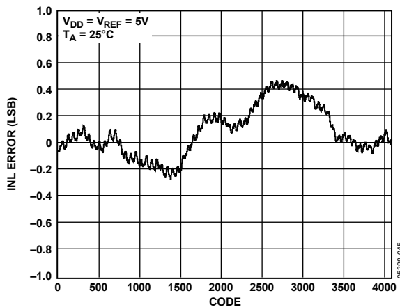
Figure 11. INL—12-Bit DAC
