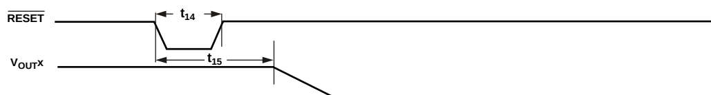
Figure 3. \overline{\text{RESET}} Timing Diagram
