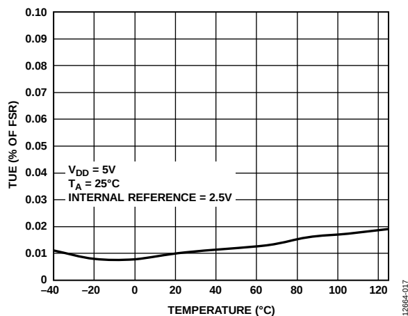
Figure 16. AD5675R TUE vs. Temperature
