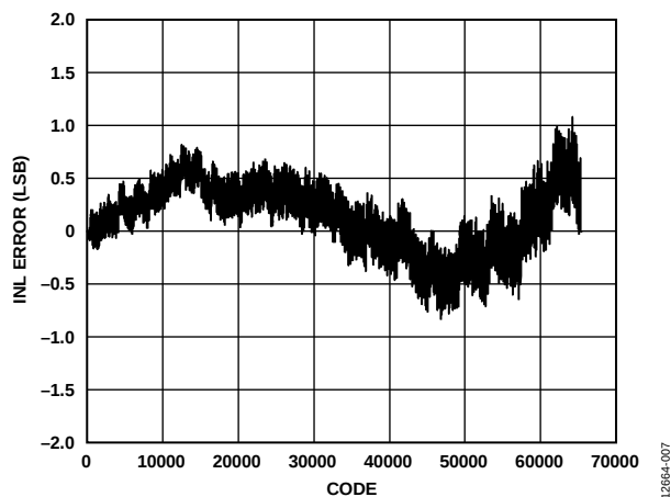
Figure 6. AD5675R INL Error vs. Code
