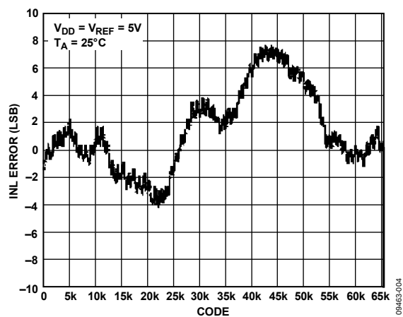
Figure 4. INL—External Reference
