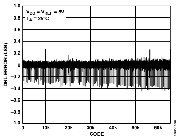
Figure 6. DNL—External Reference
