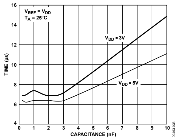
Figure 32. Settling Time vs. Capacitive Load
