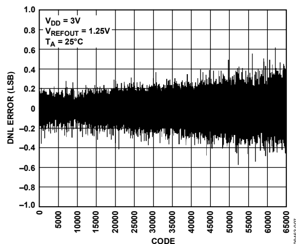
Figure 7. DNL
