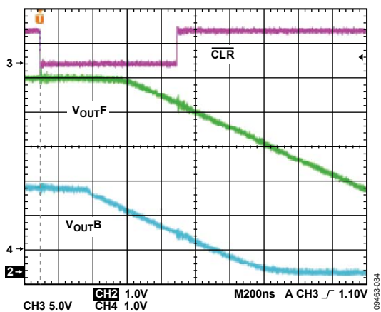
Figure 33. Hardware \overline{\text{CLR}}
