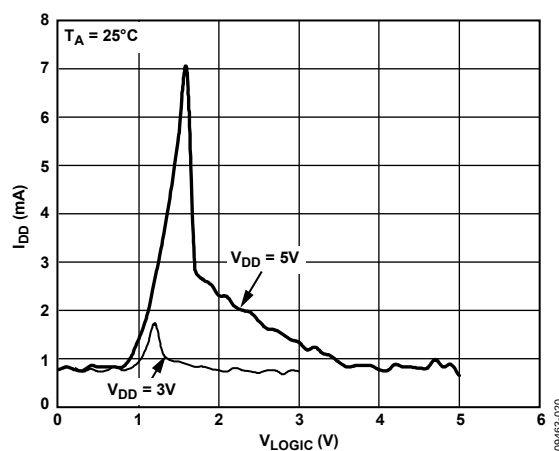
Figure 19. Supply Current ( I_{DD} ) vs. Logic Input Voltage ( V_{LOGIC} )
