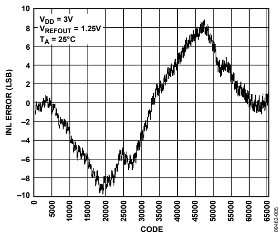
Figure 5. INL
