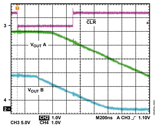
Figure 27. CLR Pulse Activation Time
