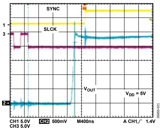
Figure 19. Exiting Power-Down to Midscale
