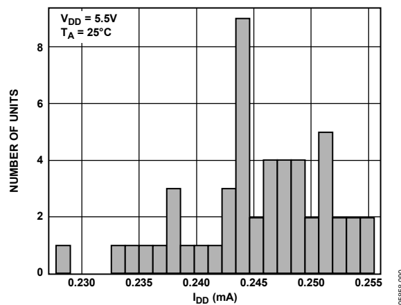
Figure 14. I_{DD} Histogram with V_{DD} = 5.5\text{ V}
