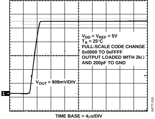
Figure 21. Full-Scale Settling Time, 5 V
