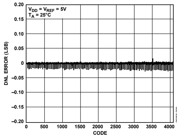
Figure 9. DNL AD5625, External Reference
