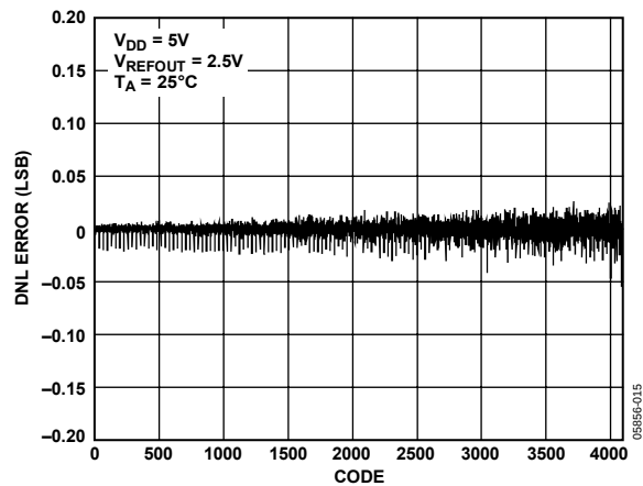
Figure 15. DNL AD5625R, 2.5V Internal Reference
