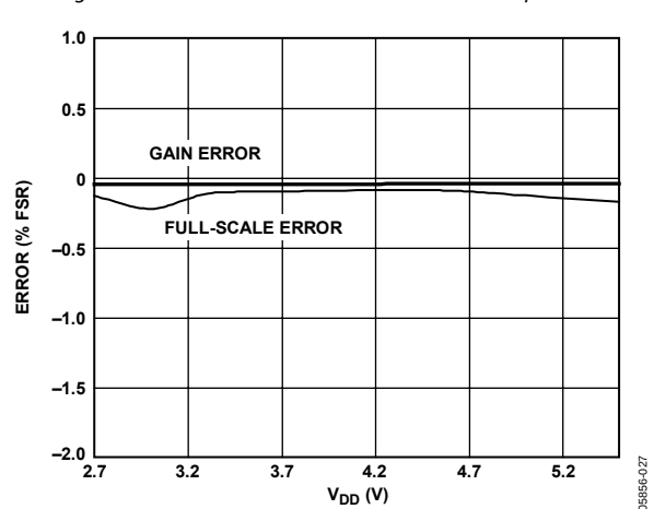
Figure 27. Gain Error and Full-Scale Error vs. Supply
