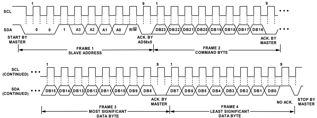
Figure 55. I²C Read Operation(14-Pin Package)
