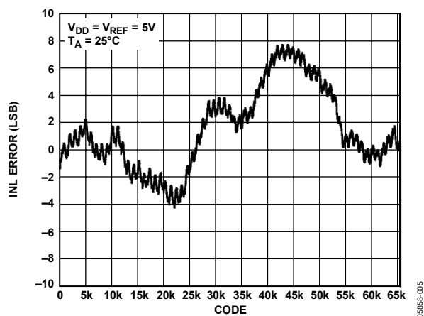
Figure 4. INL AD5665, External Reference
