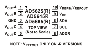
Pin Configuration (10-pin)
