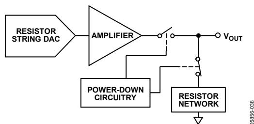
Figure 64. Output Stage During Power-Down
