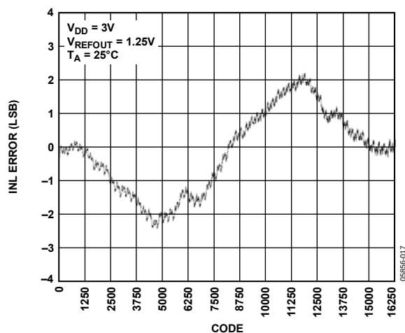
Figure 17. INL AD5645R, 1.25V Internal Reference
