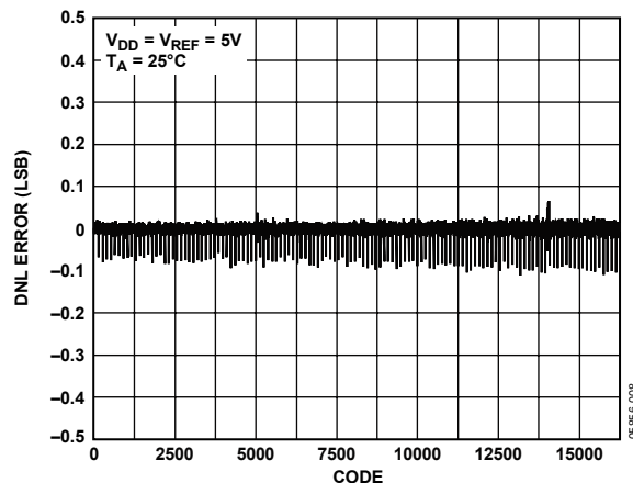
Figure 8. DNL AD5645, External Reference
