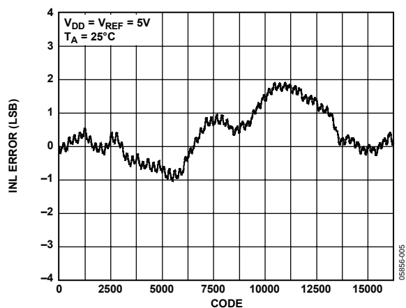
Figure 5. INL AD5645, External Reference
