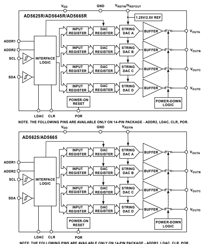
Figure 1. Functional Block Diagrams
