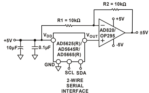
Figure 68. Bipolar Operation with the AD5625R/AD5645R/AD5665R, AD5625/AD5665
