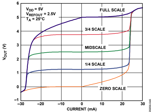
Figure 34. AD56x5R with 2.5V Reference, Source and Sink Capability
