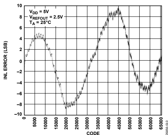
Figure 10. INL AD5665R, 2.5V Internal Reference
