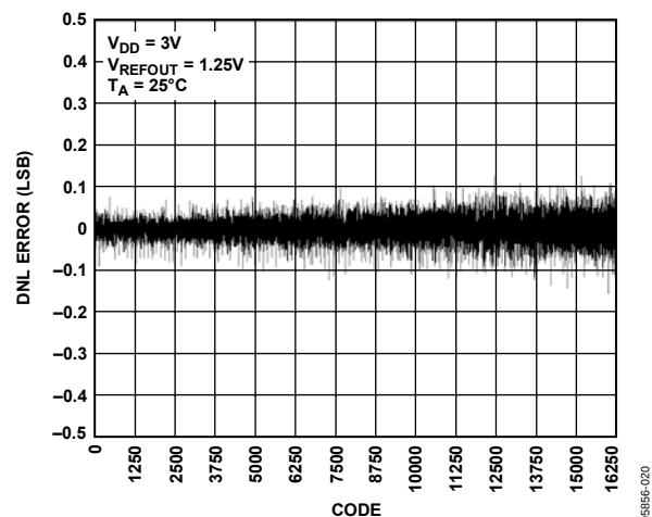
Figure 20. DNL AD5645R, 1.25V Internal Reference
