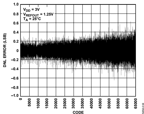
Figure 19. DNL AD5665R, 1.25V Internal Reference
