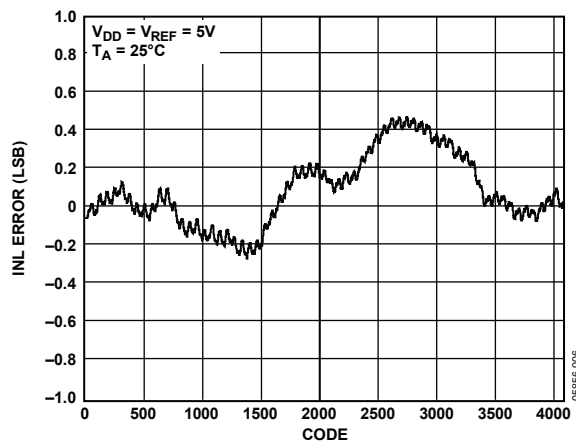
Figure 6. INL AD5625, External Reference
