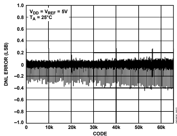
Figure 7. DNL AD5665, External Reference
