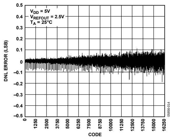
Figure 14. DNL AD5645R, 2.5V Internal Reference
