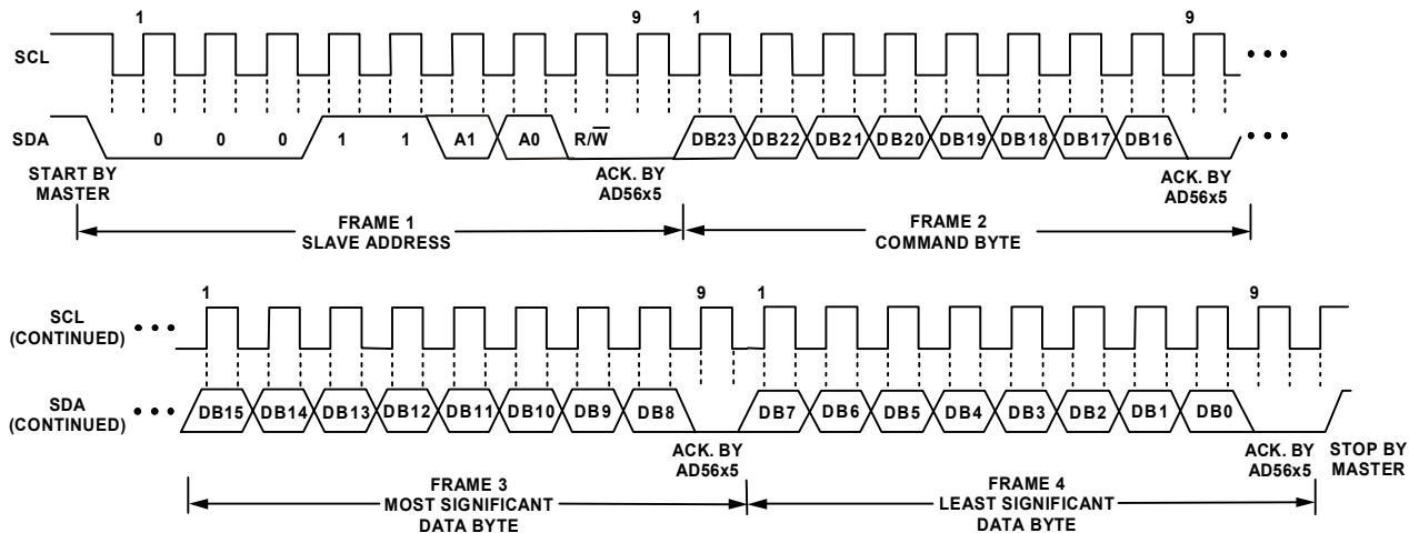
Figure 52. I²C Write Operation (10-Pin Package)
