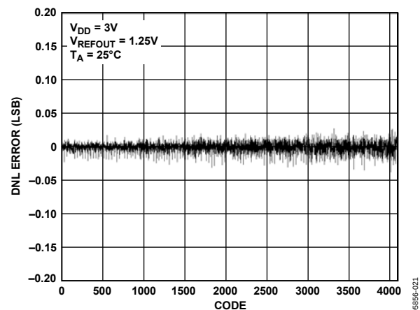
Figure 21. DNL AD5625R, 1.25V Internal Reference
