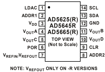
Pin Configuration (14-pin)
