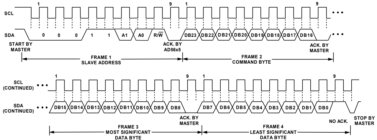
Figure 54. I²C Read Operation(10-Pin Package)
