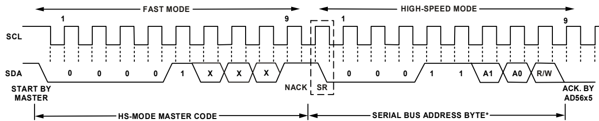
Figure 56. Placing the AD56x5 in High-Speed Mode
