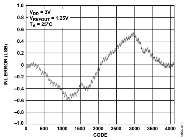
Figure 18. INL AD5625R, 1.25V Internal Reference
