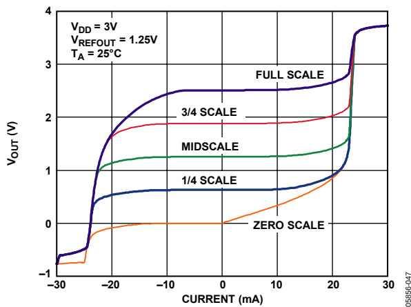
Figure 35. AD56x5R with 1.25V Reference, Source and Sink Capability
