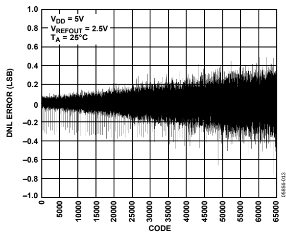
Figure 13. DNL AD5665R, 2.5V Internal Reference
