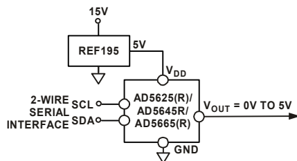
Figure 67. REF195 as Power Supply to the AD5625R/AD5645R/AD5665R, AD5625/AD5665
