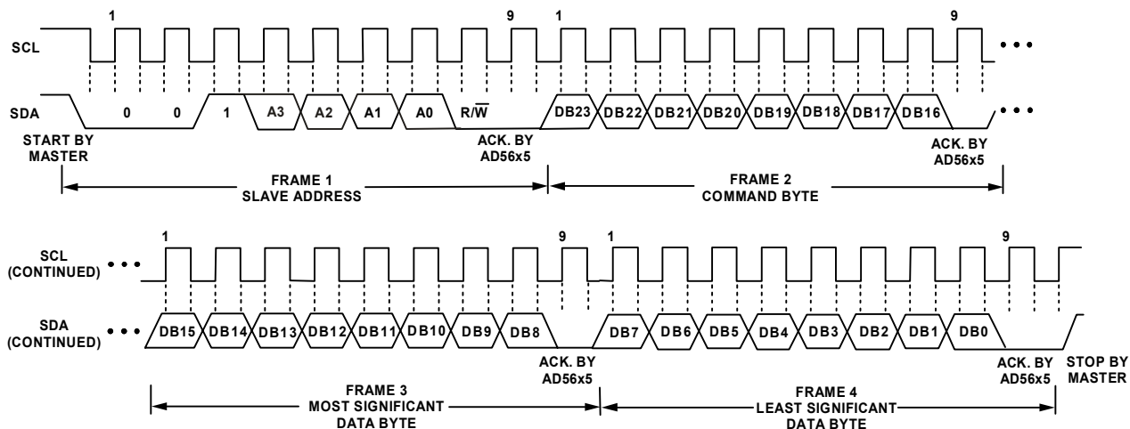
Figure 53. I²C Write Operation (14-Pin Package)
