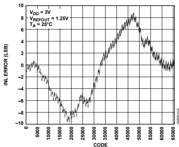
Figure 16. INL AD5665R, 1.25V Internal Reference
