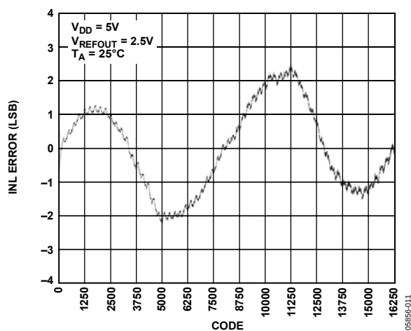
Figure 11. INL AD5645R, 2.5V Internal Reference
