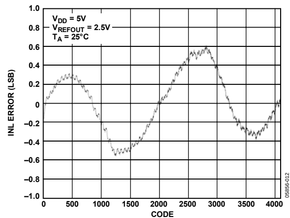
Figure 12. INL AD5625R, 2.5V Internal Reference
