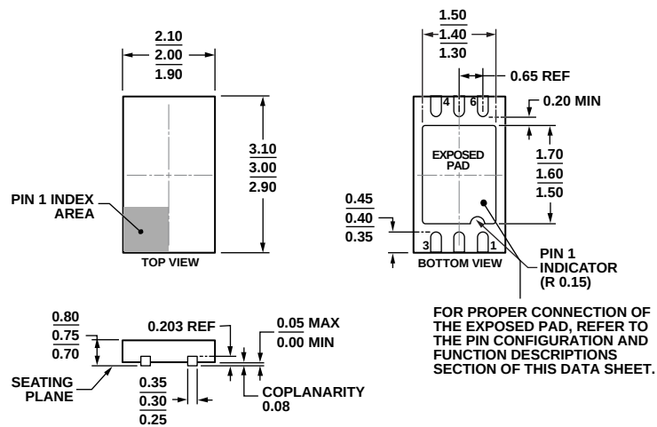
Figure 47. 6-Lead Lead Frame Chip Scale Package [LF CSP_WD] 2.00 x 3.00 mm Body, Very Very Thin, Dual Lead (CP-6-5)
