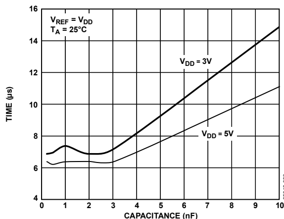
Figure 26. Settling Time vs. Capacitive Load
