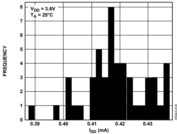
Figure 17. I_{DD} Histogram with V_{DD} = 3.6V
