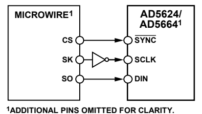
Figure 39. MICROWIRE Interface to AD5624/AD5664
