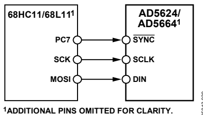
Figure 37. 68HC11/68L11 Interface to AD5624/AD5664
