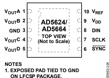
Figure 4. 10-Lead LFCSP Pin Configuration
