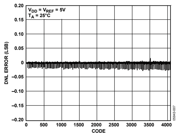
Figure 8. DNL AD5624
