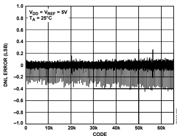
Figure 7. DNL AD5664
