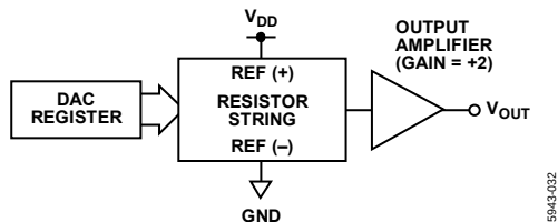
Figure 30. DAC Architecture
