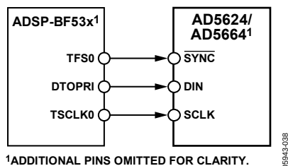
Figure 36. Blackfin ADSP-BF53x Interface to AD5624/AD5664
