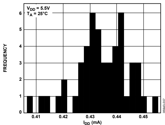
Figure 16. I_{DD} Histogram with V_{DD} = 5.5V
