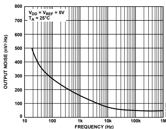
Figure 28. Noise Spectral Density
