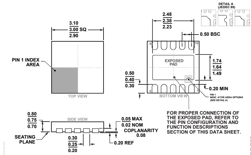
Figure 43. 10-Lead Lead Frame Chip Scale Package [LFCSP] 3 mm × 3 mm Body and 0.75 mm Package Height (CP-10-9)
