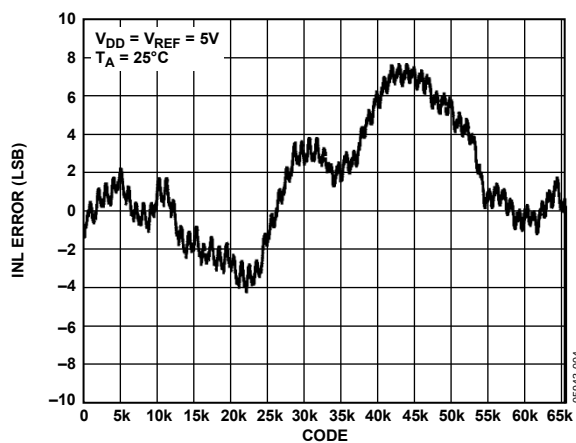
Figure 5. INL AD5664
