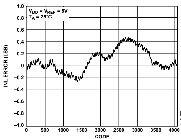
Figure 6. INL AD5624
