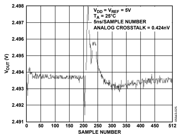
Figure 24. Analog Crosstalk
