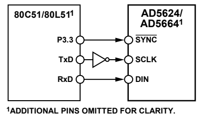
Figure 38. 80C51/80L51 Interface to AD5624/AD5664
