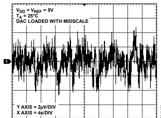
Figure 27. 0.1 Hz to 10 Hz Output Noise Plot
