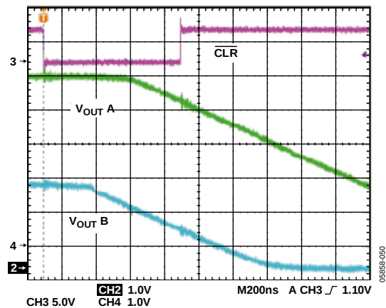
Figure 48. \overline{\text{CLR}} Pulse Activation Time
