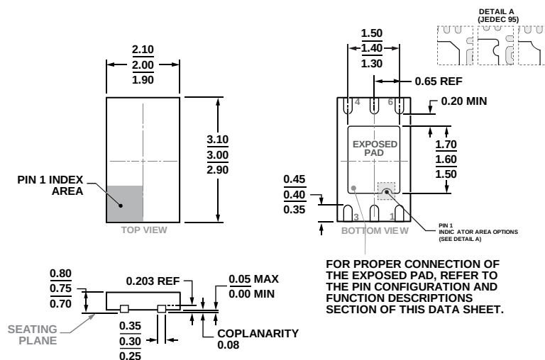
Figure 53. 6-Lead Lead Frame Chip Scale Package [LFCSP] 2.00 mm x 3.00 mm Body and 0.75 mm Package Height (CP-6-5)
