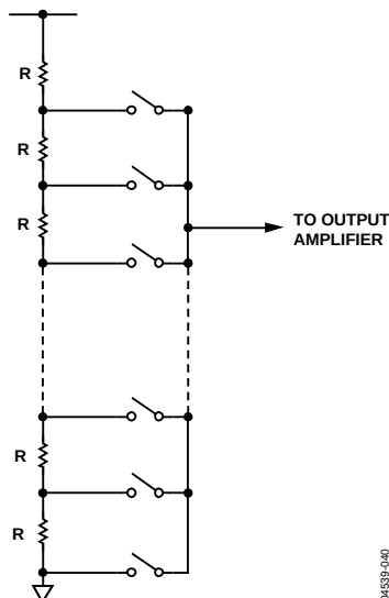
Figure 39. Resistor String
