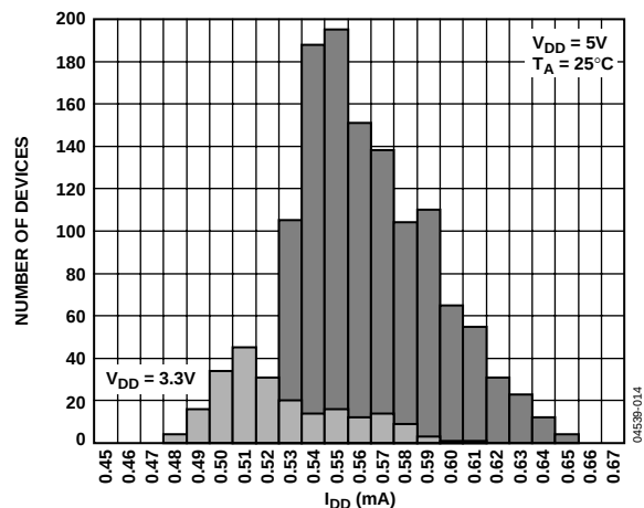
Figure 20. I_{DD} Histogram
