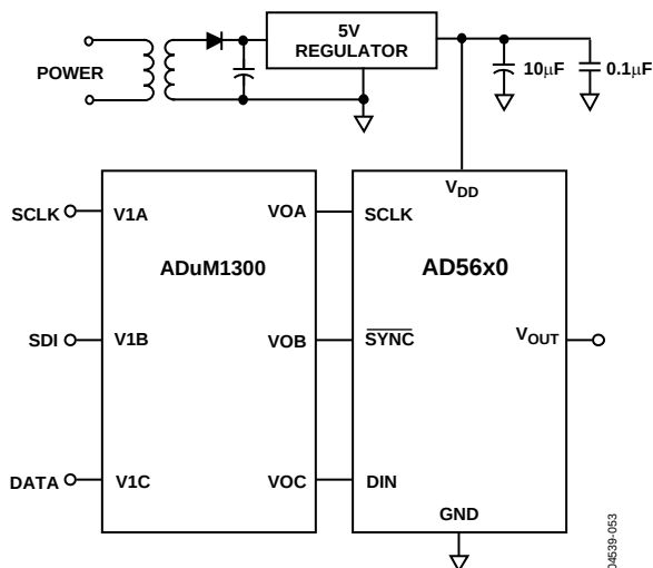
Figure 52. AD5620/AD5640/AD5660 with a Galvanically Isolated Interface
