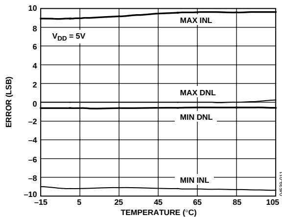
Figure 17. INL Error and DNL Error vs. Temperature
