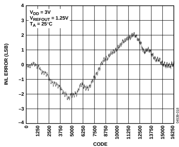
Figure 12. INL—AD5640-1
