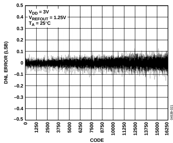
Figure 15. DNL—AD5640-1
