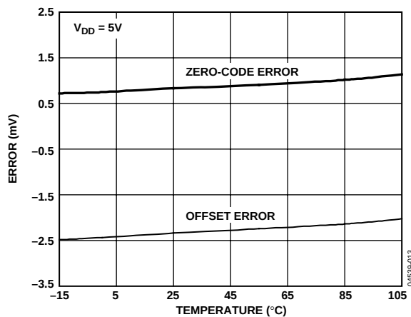
Figure 19. Zero-Code and Offset Error vs. Temperature
