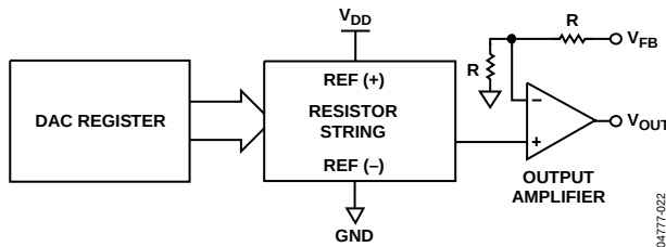
Figure 38. DAC Architecture
