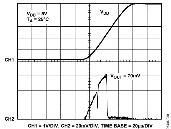
Figure 27. Power-On Reset to 0 V
