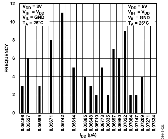
Figure 25. I_{DD} Histogram (3 V/5 V Supply)
