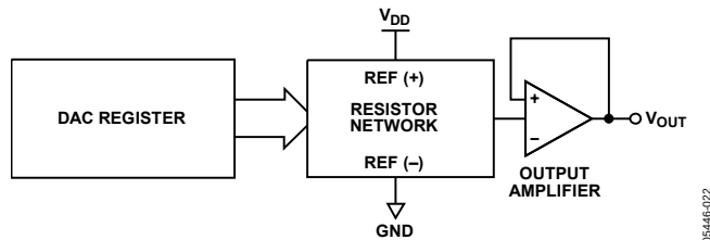
Figure 36. DAC Architecture
