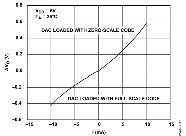
Figure 26. Sink and Source Capability
