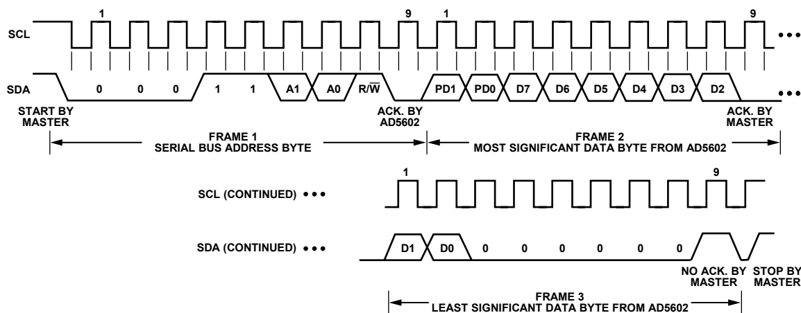
Figure 45. AD5602 Read Sequence
