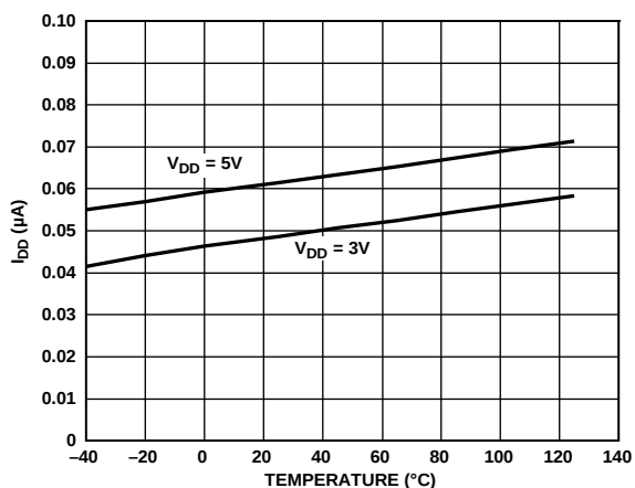
Figure 23. Supply Current vs. Temperature (3 V/5 V Supply)
