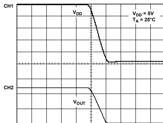
Figure 32. V_{OUT} vs. V_{DD}
