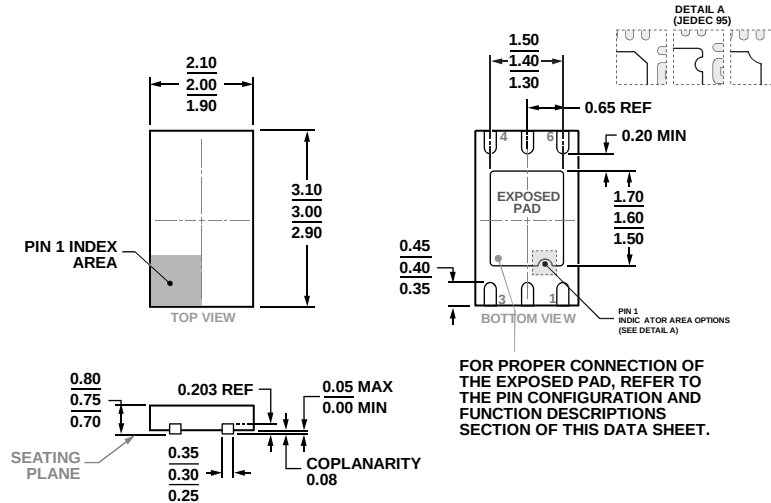
Figure 53. 6-Lead Lead Frame Chip Scale Package [LFCSP] 2.00 mm x 3.00 mm Body and 0.75 mm Package Height (CP-6-5)
