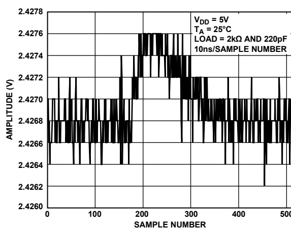
Figure 34. Digital Feedthrough
