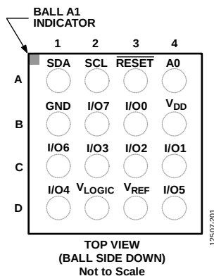
Figure 5. 16-Ball WLCSP Pin Configuration
