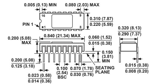
16-Lead Side-Brazed Ceramic Dual In-Line Package [SBDIP] (D-16) Dimensions shown in inches and (millimeters)
