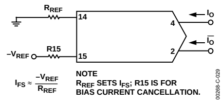
Figure 28. Basic Negative Reference Operation
