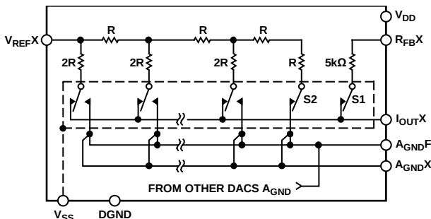
DIGITAL INTERFACE CONNECTIONS OMITTED FOR CLARITY. SWITCHES S1 AND S2 ARE CLOSED, AND V_{\text{DD}} MUST BE POWERED.
