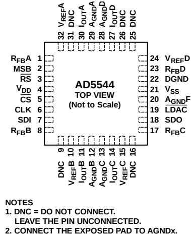
Figure 6. LFCSP Pin Configuration
