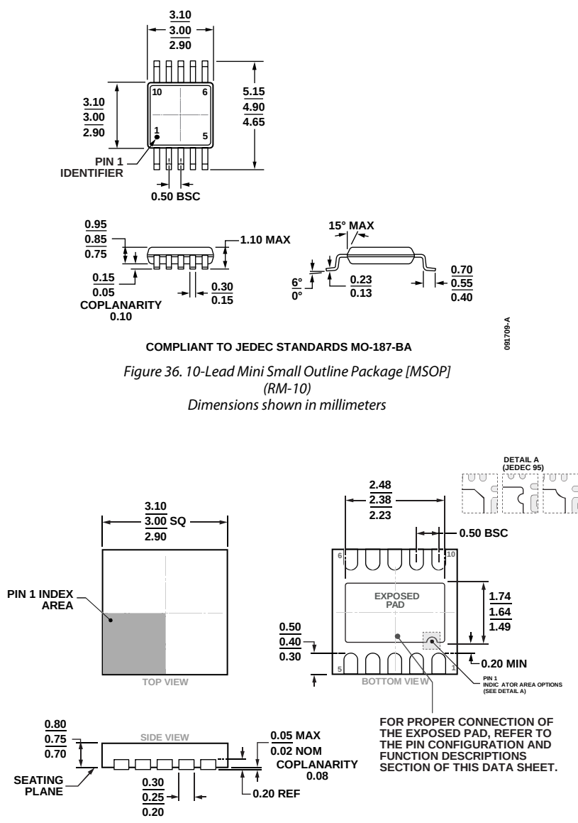
Figure 37. 10-Lead Lead Frame Chip Scale Package [LFCSP] 3 mm × 3 mm Body and 0.75 mm Package Height (CP-10-9)
