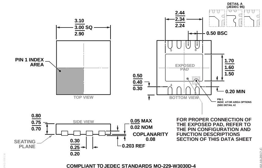
Figure 38. 8-Lead Lead Frame Chip Scale Package [LFCSP]
