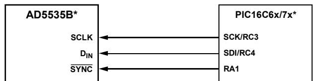
Figure 18. AD5535B-to-PIC16C6x/7x Interface
