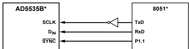
Figure 19. AD5535B-to-8051 Interface
