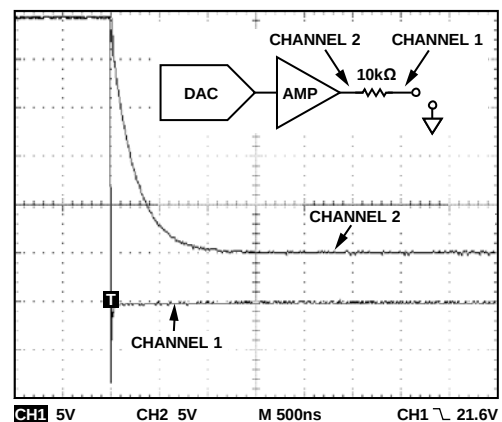
Figure 8. Short-Circuit Current Limit Timing
