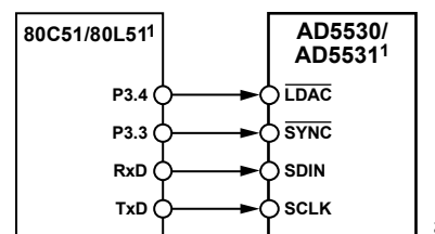
Figure 24. AD5530/AD5531 to 8051 Interface
