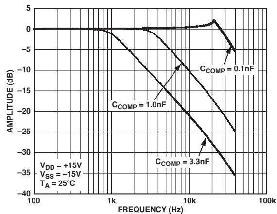
TPC 6. Force Amplifier Bandwidth—MODE 1 (40 \mu A )
