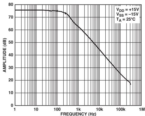
TPC 2. Voltage Sense Amplifier CMRR vs. Frequency
