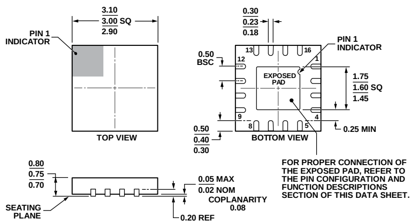
Figure 39. 16-Lead Lead Frame Chip Scale Package [LFCSP_WQ] 3 mm × 3 mm Body, Very Very Thin Quad (CP-16-22)
