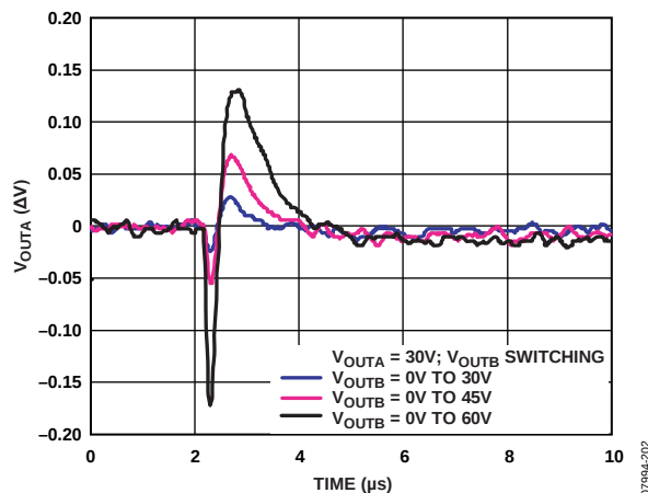
Figure 15. DAC-to-DAC Crosstalk
