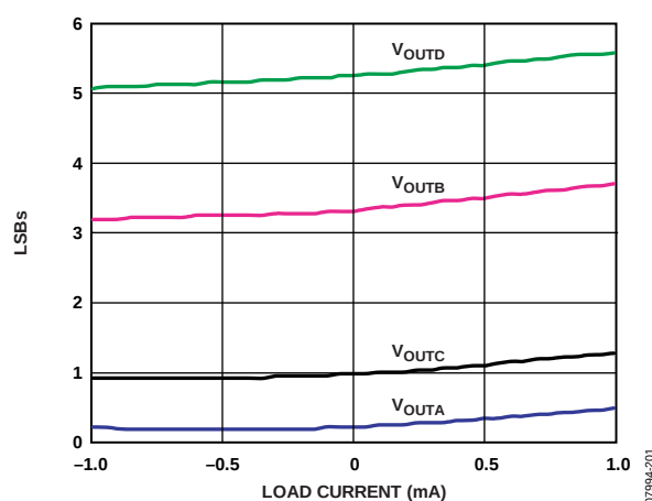
Figure 16. DAC-to-DAC Mismatch
