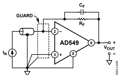
Figure 28. Inverting Amplifier with Guard
