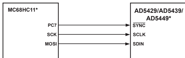
Figure 53. MCH68HC11/68L11-to-AD5429/AD5439/AD5449 Interface
