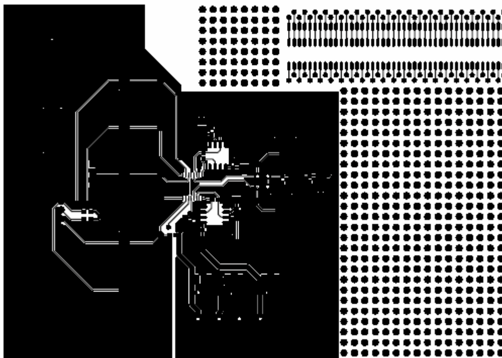
Figure 57. Component-Side Artwork
