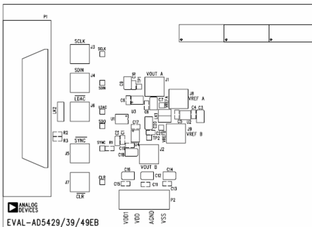
Figure 58. Silkscreen—Component-Side View (Top)
