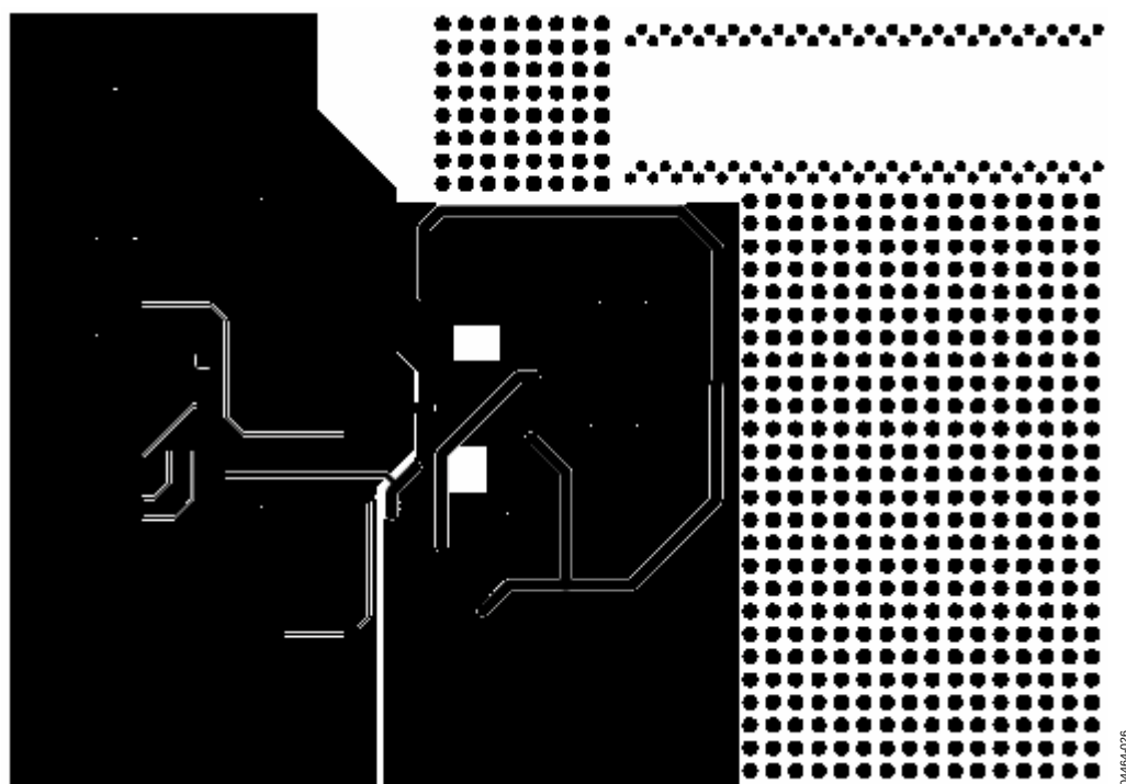
Figure 59. Solder-Side Artwork
