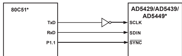
Figure 51. 80C51/80L51-to-AD5429/AD5439/AD5449 Interface
