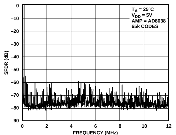
Figure 29. Wideband SFDR, f_{OUT} = 100\text{ kHz} , Clock = 25 MHz
