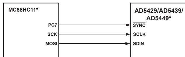
Figure 52. MCH68HC11/68L11-to-AD5429/AD5439/AD5449 Interface
