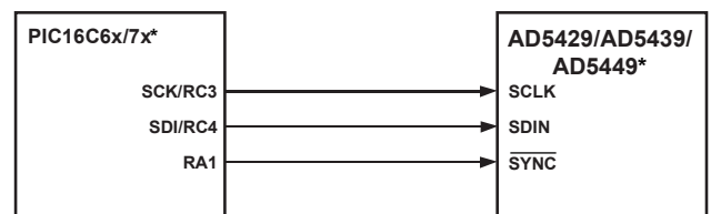
Figure 54. PIC16C6x/7x-to-AD5429/AD5439/AD5449 Interface
