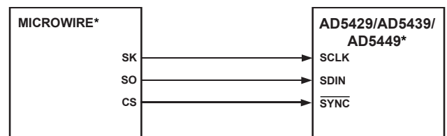
Figure 53. MICROWIRE-to-AD5429/AD5439/AD5449 Interface
