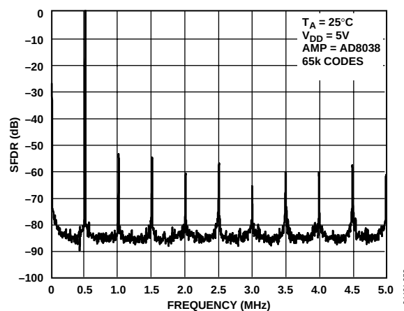
Figure 30. Wideband SFDR, f_{OUT} = 500\text{ kHz} , Clock = 10 MHz
