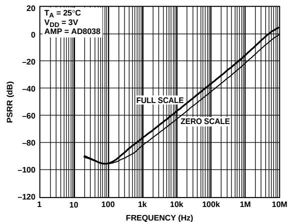
Figure 25. Power Supply Rejection Ratio vs. Frequency
