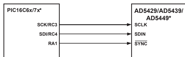
Figure 54. PIC16C6x/7x-to-AD5429/AD5439/AD5449 Interface
