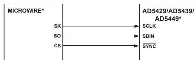
Figure 53. MICROWIRE-to-AD5429/AD5439/AD5449 Interface
