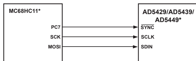
Figure 52. MCH68HC11/68L11-to-AD5429/AD5439/AD5449 Interface
