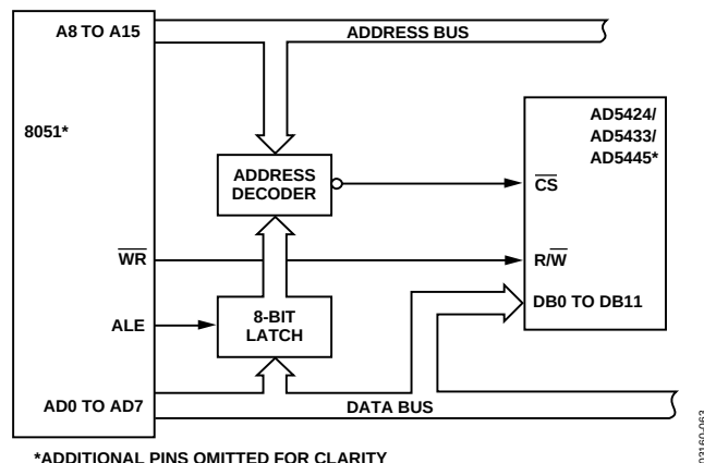
Figure 56. 8xC51-to-AD5424/AD5433/AD5445 Interface
