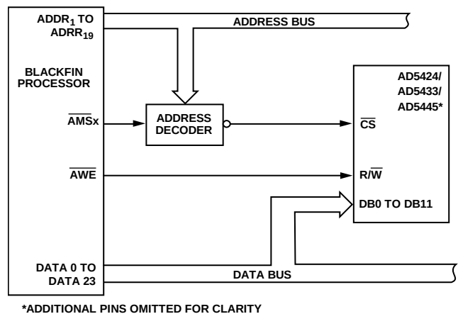
Figure 57. Blackfin Processor-to-AD5424/AD5433/AD5445 Interface
