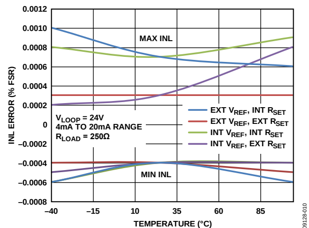
Figure 12. Integral Nonlinearity Error vs. Temperature
