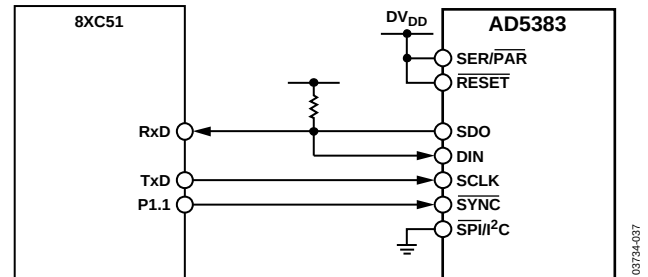
Figure 37. AD5383-to-8051 Interface
