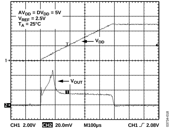
Figure 18. Power-Up Transient
