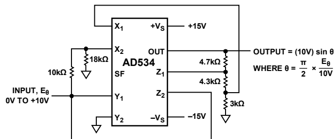
Figure 21. Voltage-Controlled Amplifier
